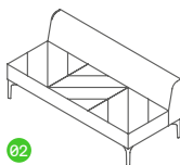
02 HAT3NA hatch 3 seater no arms metric (mm) W1530 D690 H685 Seat 410 imperial (in) W60 D27 H27 Seat 16
