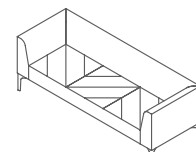
HAT32A hatch 3 seater 2 arms metric (mm) W1890 D690 H685 Seat 410 imperial (in) W74.5 D27 H27 Seat 16
