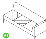
01 HAT3LA hatch 3 seater left arm metric (mm) W1710 D690 H685 Seat 410 imperial (in) W67.5 D27 H27 Seat 16
