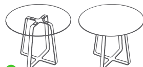
FRG850D Frog table 850 circular metric (mm) 850Dia H750 imperial (in) 33.5Dia H29.5
